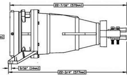
LINE MOUNTED SOCKET
